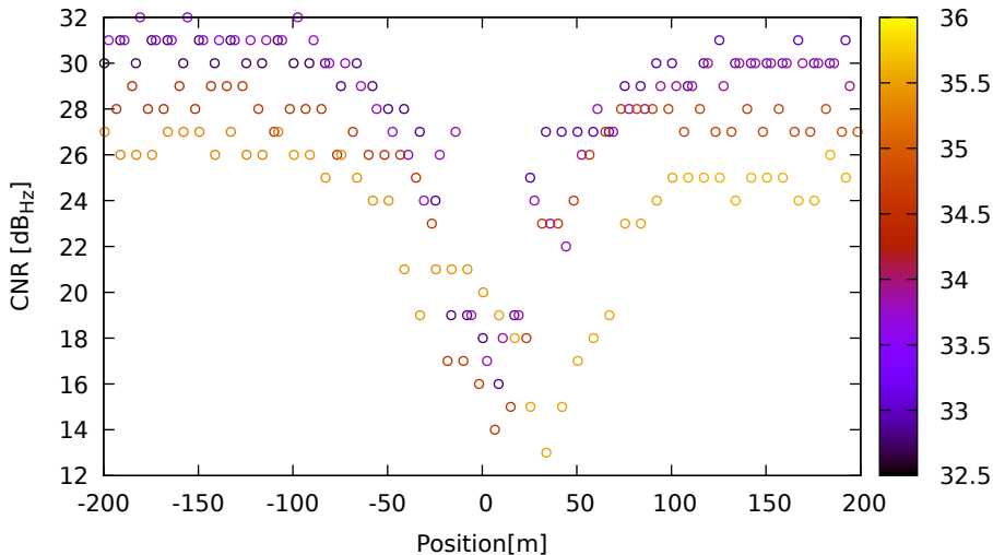
CNR vs position for G04 (L5) on HuaweiP40 - DOY 263 jam. 1
