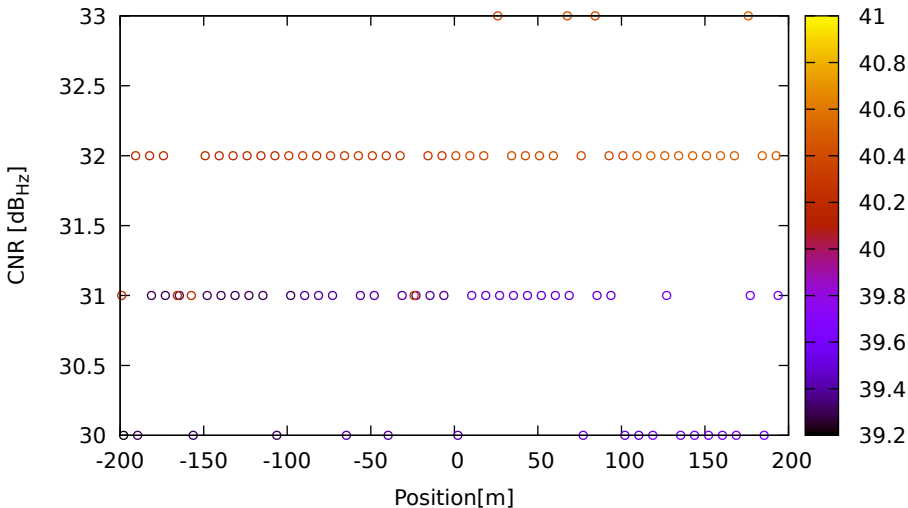
CNR vs position for G04 (L5) on HuaweiP40 - DOY 263 jam. 3
