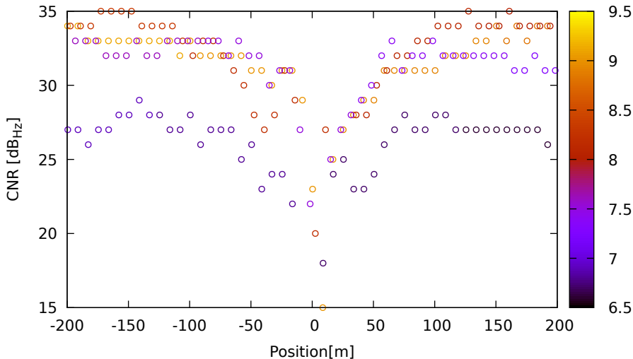
CNR vs position for G08 (L1) on HuaweiP40 - DOY 263 jam. 1
