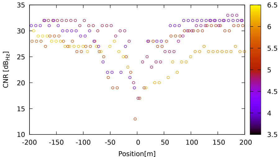
CNR vs position for G08 (L1) on HuaweiP40 - DOY 263 jam. 2
