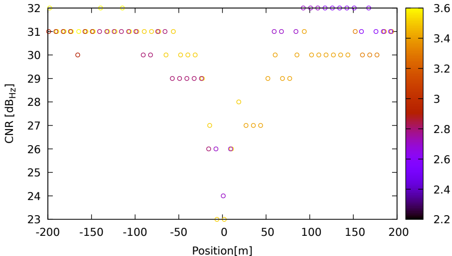
CNR vs position for G08 (L1) on HuaweiP40 - DOY 263 jam. 3
