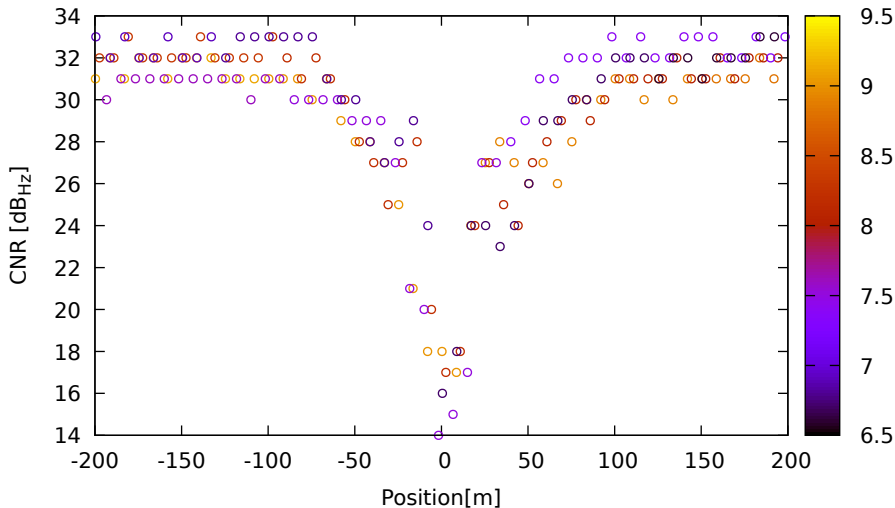
CNR vs position for G08 (L5) on HuaweiP40 - DOY 263 jam. 1
