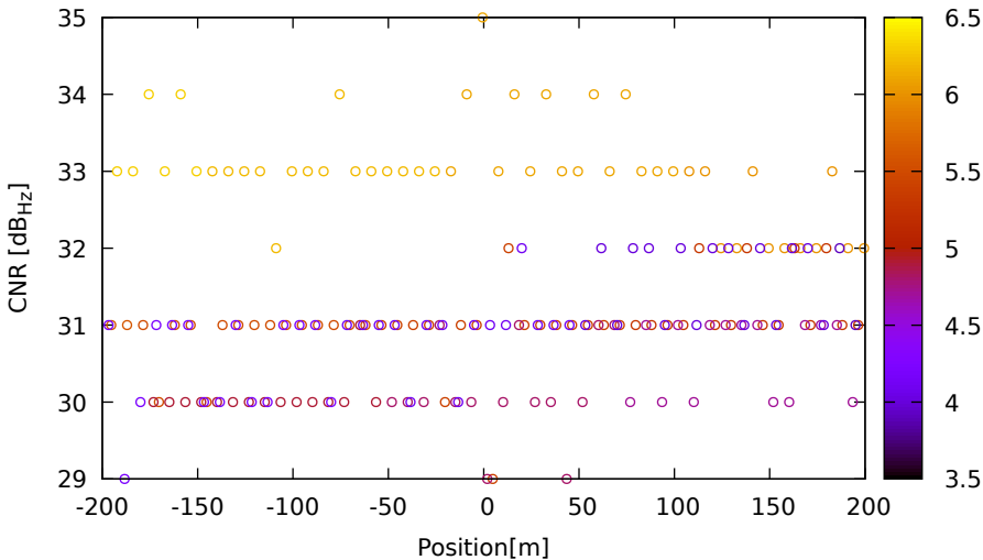
CNR vs position for G08 (L5) on HuaweiP40 - DOY 263 jam. 2
