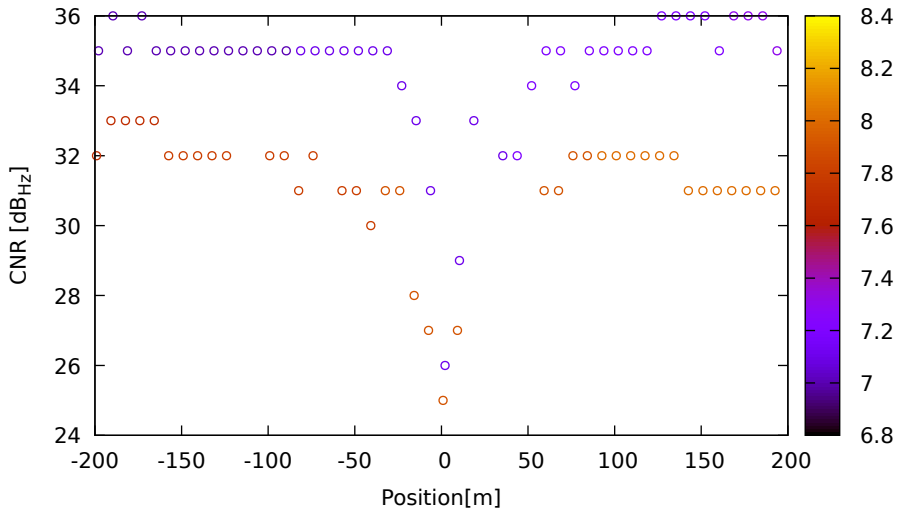
CNR vs position for G09 (L1) on HuaweiP40 - DOY 263 jam. 3
