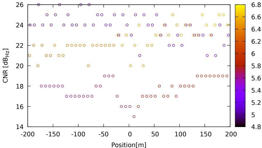
CNR vs position for G09 (L5) on HuaweiP40 - DOY 263 jam. 2
