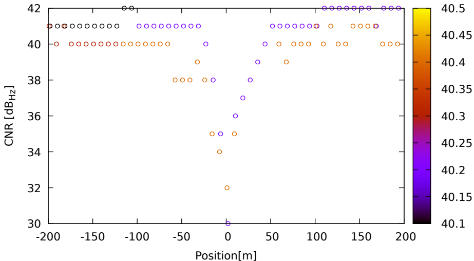
CNR vs position for G17 (L1) on HuaweiP40 - DOY 263 jam. 3
