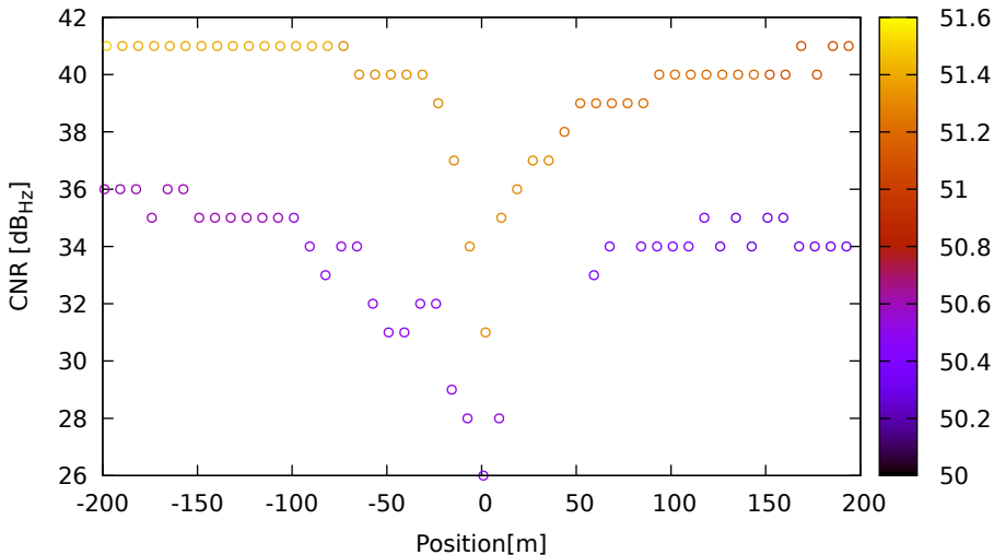
CNR vs position for G21 (L1) on HuaweiP40 - DOY 263 jam. 3
