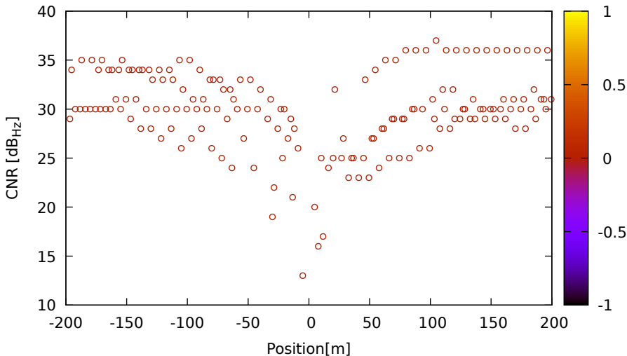
CNR vs position for G28 (L1) on HuaweiP40 - DOY 263 jam. 2
