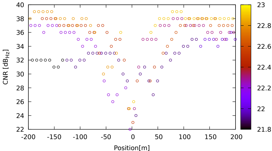
CNR vs position for G31 (L1) on HuaweiP40 - DOY 263 jam. 2
