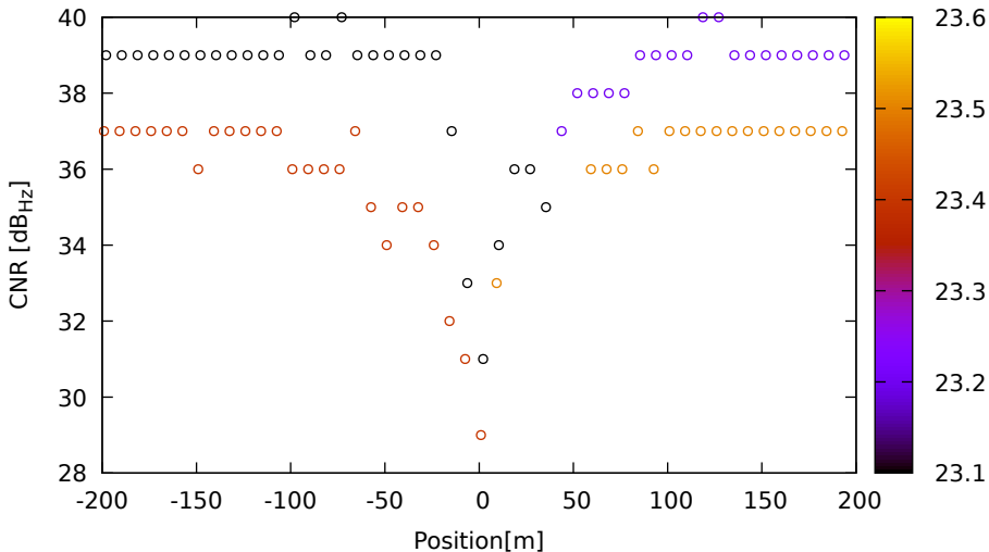
CNR vs position for G31 (L1) on HuaweiP40 - DOY 263 jam. 3
