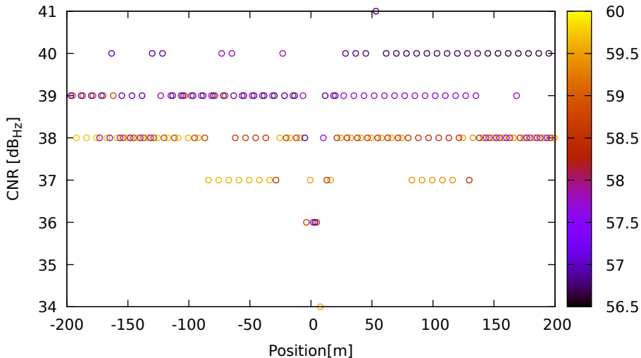
CNR vs position for R01 (G1) on HuaweiP40 - DOY 263 jam. 2
