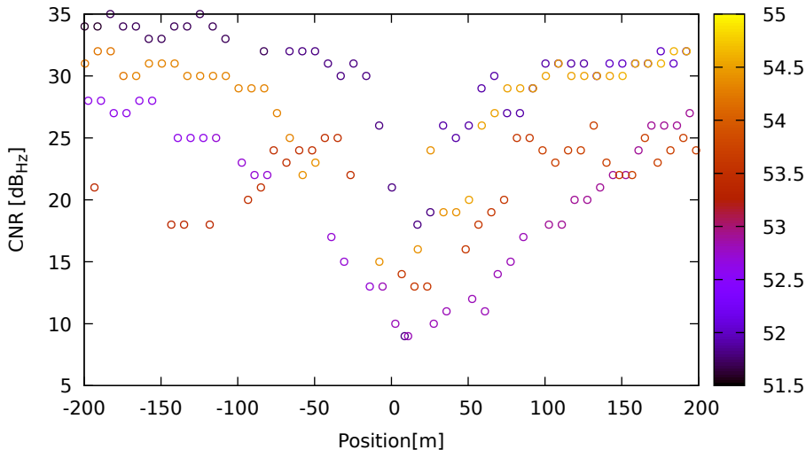
CNR vs position for R02 (G1) on HuaweiP40 - DOY 263 jam. 1
