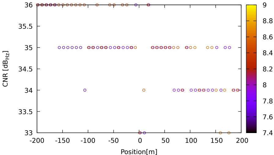
CNR vs position for R03 (G1) on HuaweiP40 - DOY 263 jam. 3
