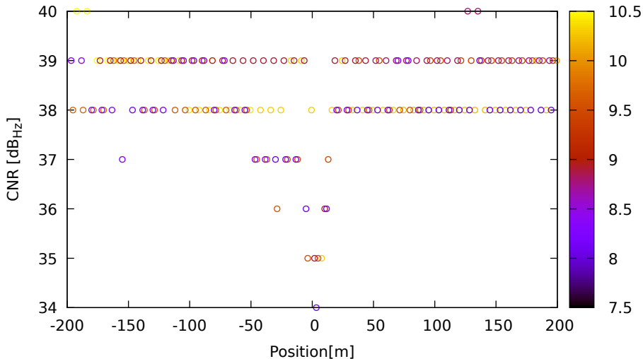
CNR vs position for R08 (G1) on HuaweiP40 - DOY 263 jam. 2
