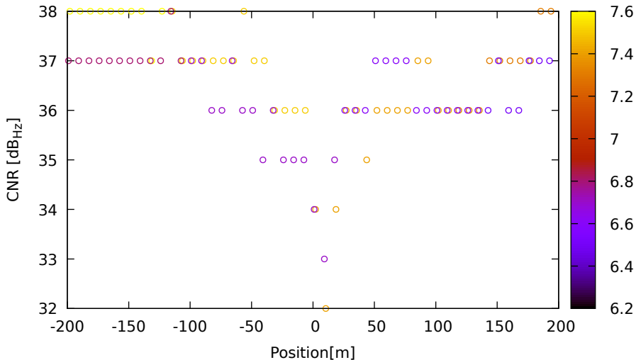
CNR vs position for R08 (G1) on HuaweiP40 - DOY 263 jam. 3
