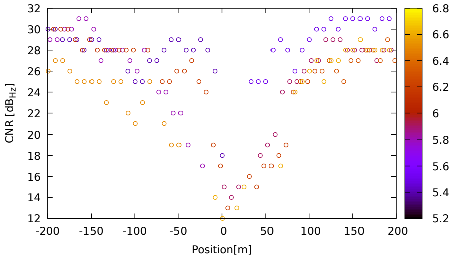
CNR vs position for R10 (G1) on HuaweiP40 - DOY 263 jam. 1
