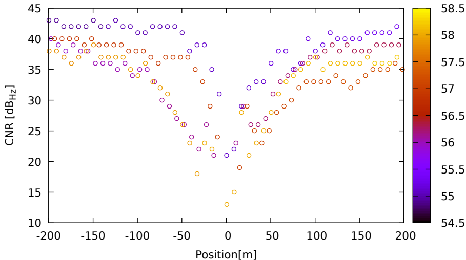
CNR vs position for R17 (G1) on HuaweiP40 - DOY 263 jam. 1
