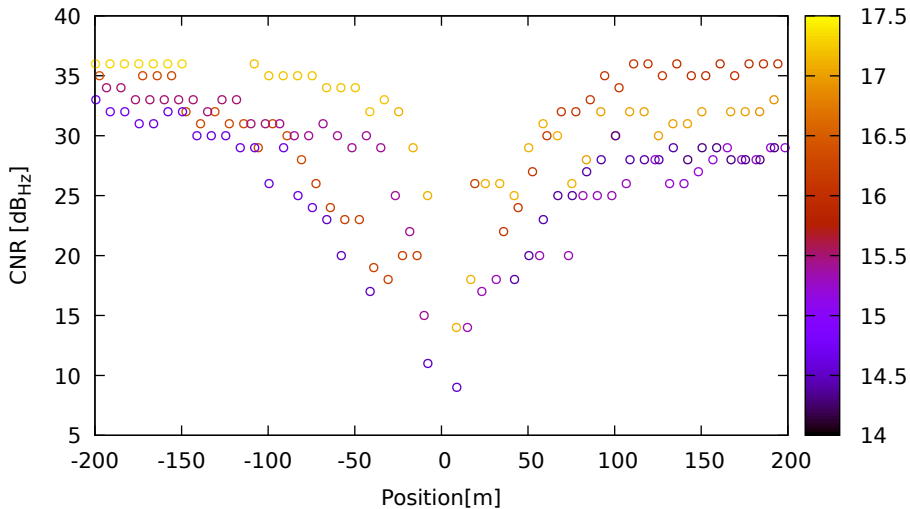
CNR vs position for R23 (G1) on HuaweiP40 - DOY 263 jam. 1
