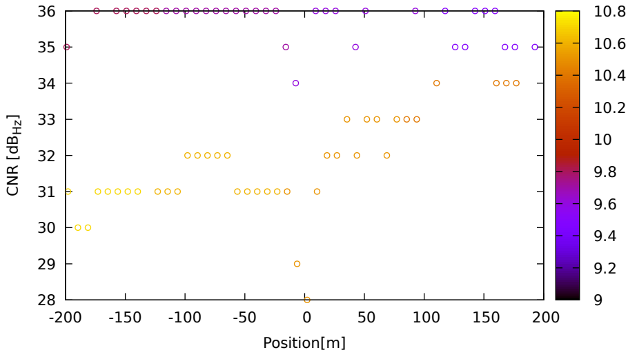
CNR vs position for R23 (G1) on HuaweiP40 - DOY 263 jam. 3
