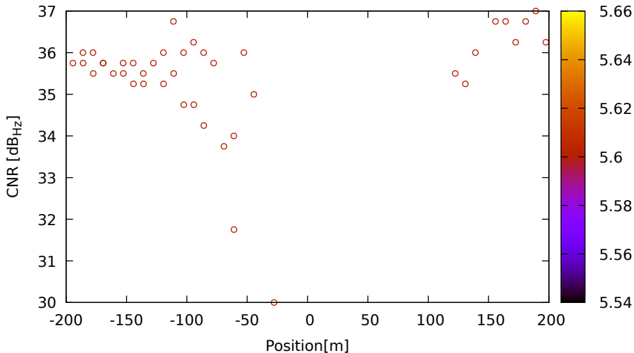
CNR vs position for C02 (B1) on LeicaGS18 - DOY 263 jam. 3
