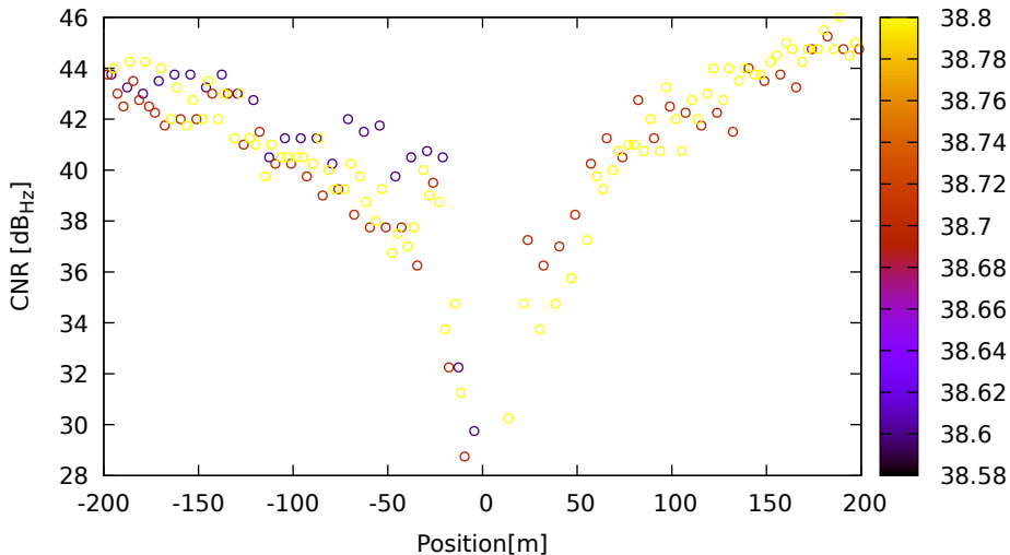
CNR vs position for C09 (B1) on LeicaGS18 - DOY 263 jam. 1
