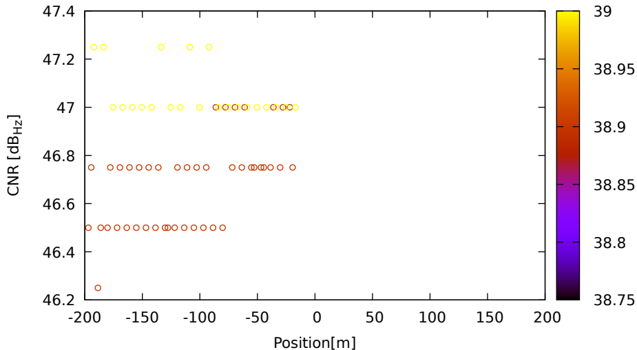
CNR vs position for C09 (B2) on LeicaGS18 - DOY 263 jam. 2
