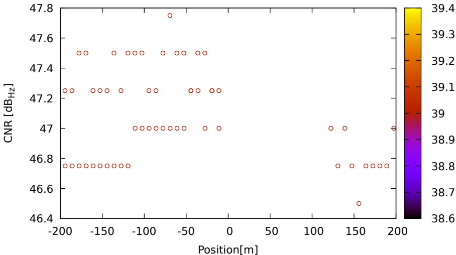
CNR vs position for C09 (B2) on LeicaGS18 - DOY 263 jam. 3
