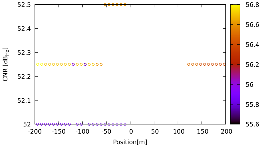
CNR vs position for C11 (B2) on LeicaGS18 - DOY 263 jam. 3
