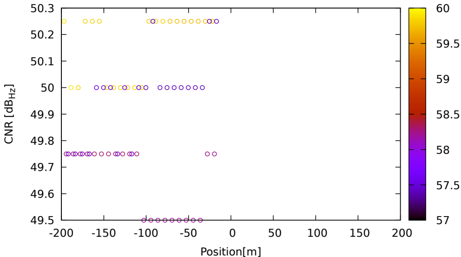
CNR vs position for C11 (B3) on LeicaGS18 - DOY 263 jam. 2
