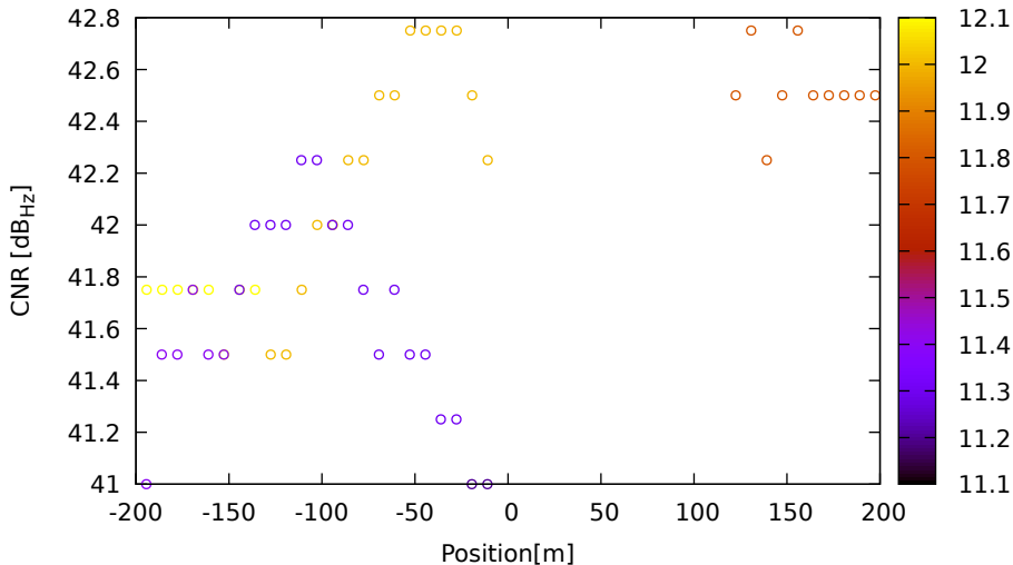
CNR vs position for C12 (B2) on LeicaGS18 - DOY 263 jam. 3
