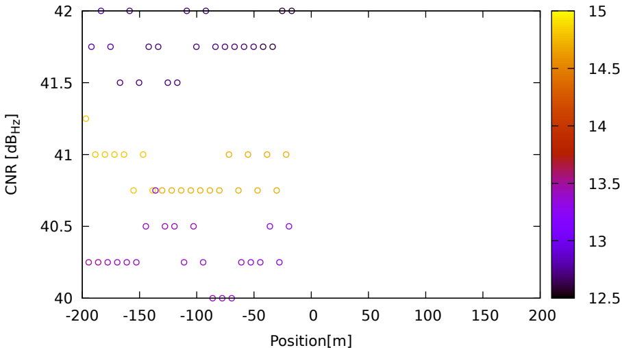
CNR vs position for C12 (B3) on LeicaGS18 - DOY 263 jam. 2
