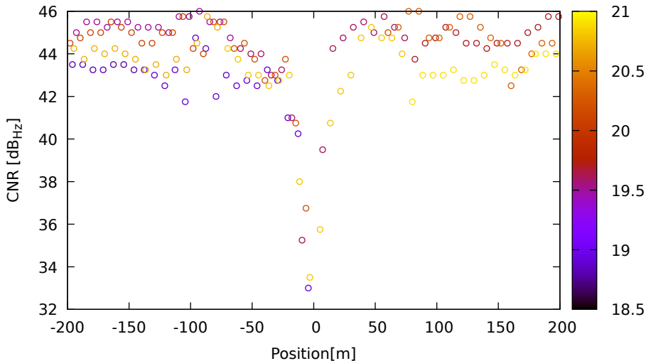
CNR vs position for C28 (B3) on LeicaGS18 - DOY 263 jam. 1
