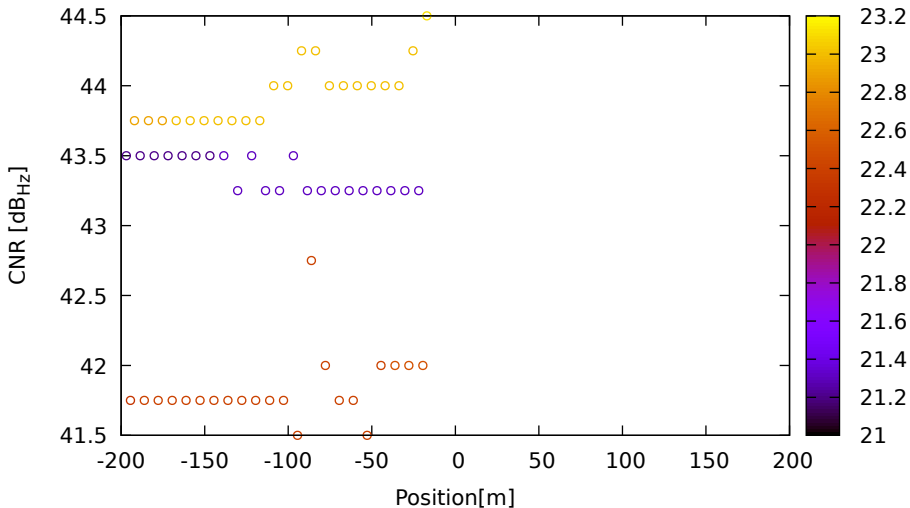
CNR vs position for C28 (B3) on LeicaGS18 - DOY 263 jam. 2
