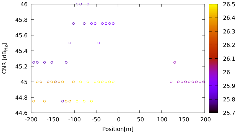
CNR vs position for C33 (B3) on LeicaGS18 - DOY 263 jam. 3
