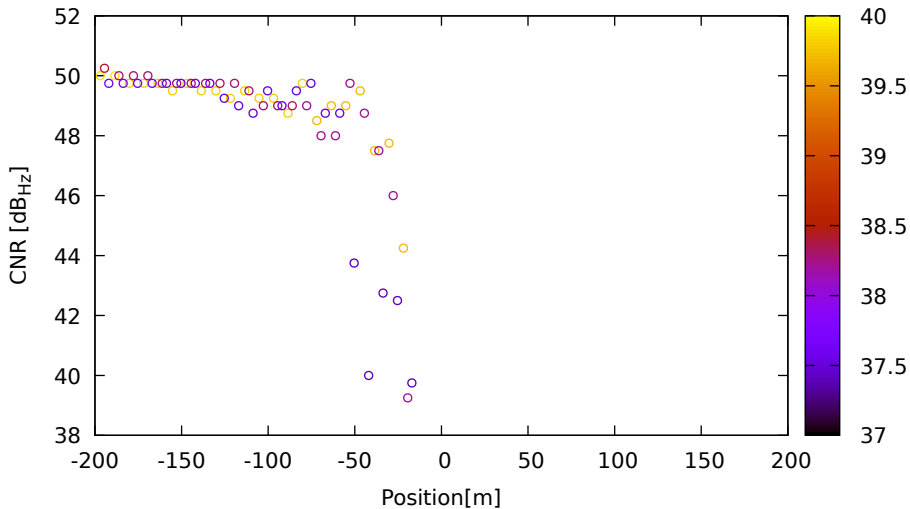
CNR vs position for C34 (B1) on LeicaGS18 - DOY 263 jam. 2
