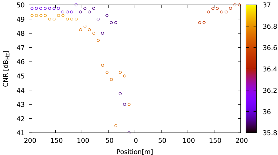
CNR vs position for C34 (B1) on LeicaGS18 - DOY 263 jam. 3
