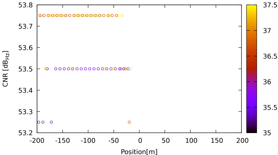
CNR vs position for E04 (E5) on LeicaGS18 - DOY 263 jam. 2
