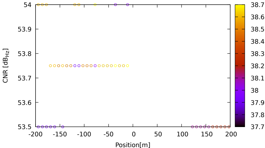
CNR vs position for E04 (E5) on LeicaGS18 - DOY 263 jam. 3
