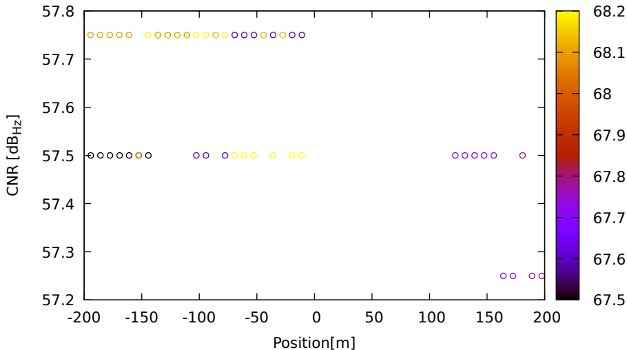
CNR vs position for E10 (E5) on LeicaGS18 - DOY 263 jam. 3
