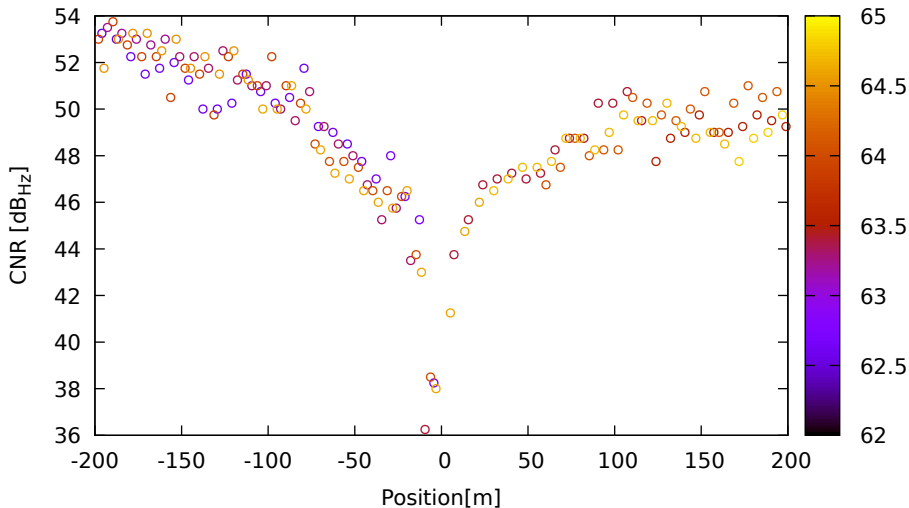
CNR vs position for E10 (E5a) on LeicaGS18 - DOY 263 jam. 1
