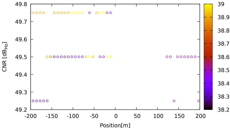
CNR vs position for E11 (E5) on LeicaGS18 - DOY 263 jam. 3
