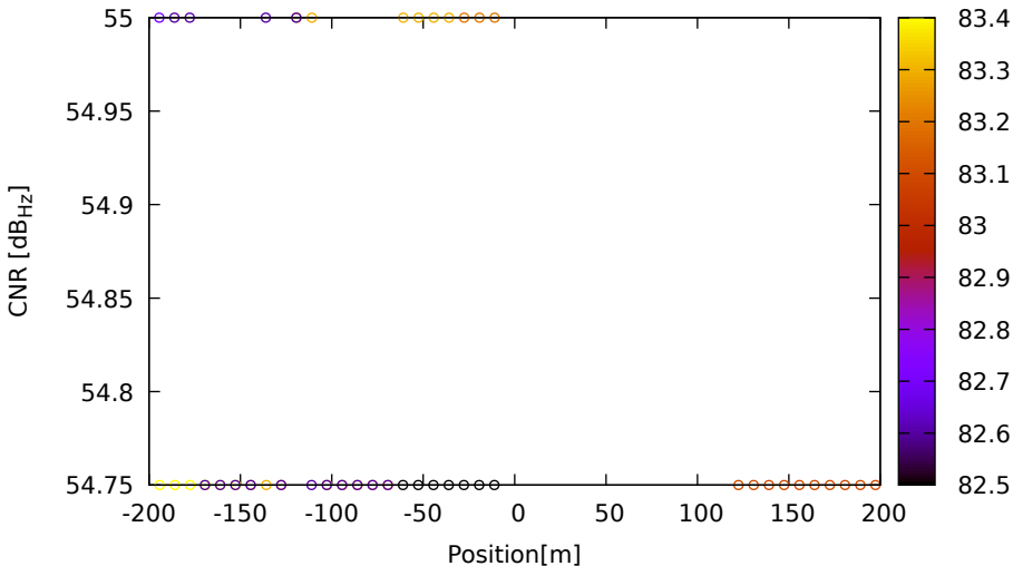
CNR vs position for E12 (E5) on LeicaGS18 - DOY 263 jam. 3
