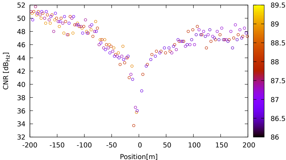
CNR vs position for E12 (E5a) on LeicaGS18 - DOY 263 jam. 1
