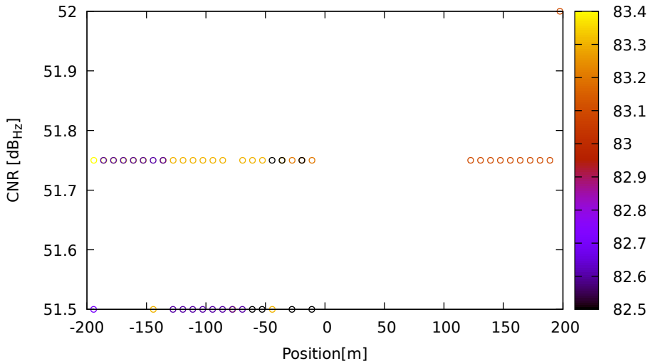
CNR vs position for E12 (E5a) on LeicaGS18 - DOY 263 jam. 3
