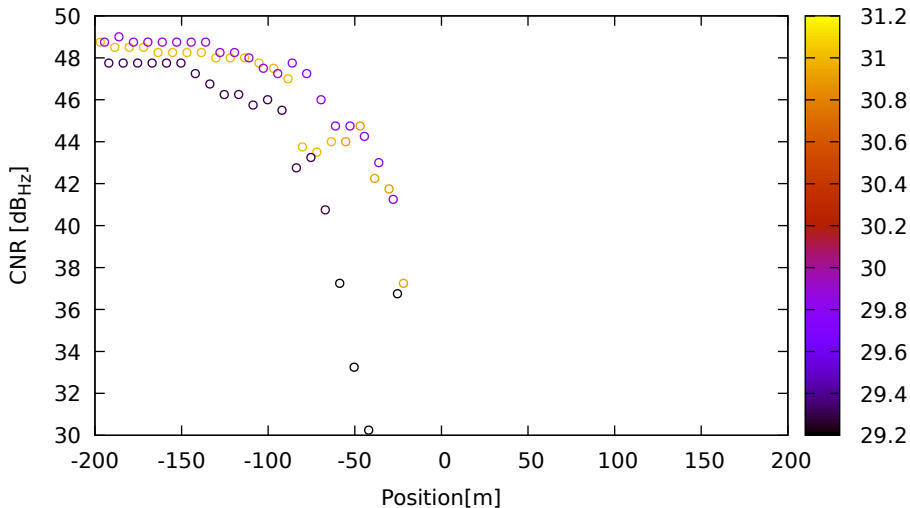
CNR vs position for E33 (E1) on LeicaGS18 - DOY 263 jam. 2
