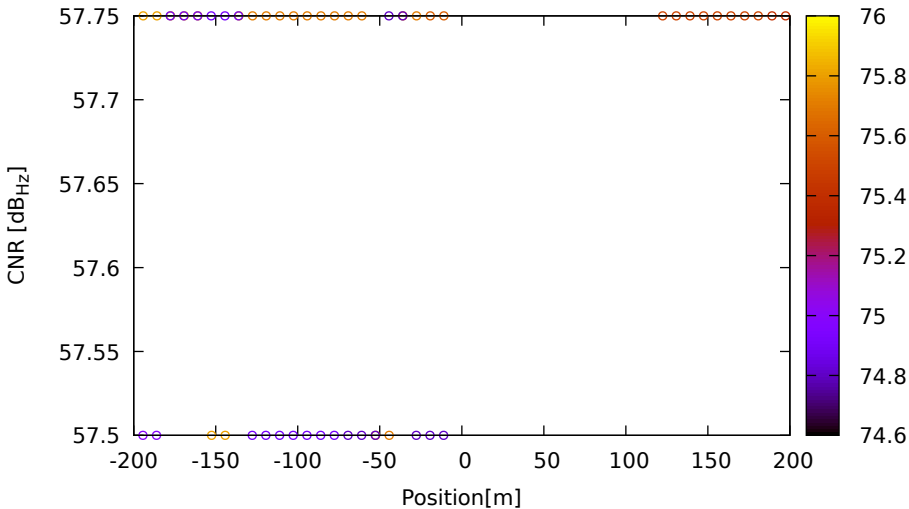
CNR vs position for G01 (L5) on LeicaGS18 - DOY 263 jam. 3
