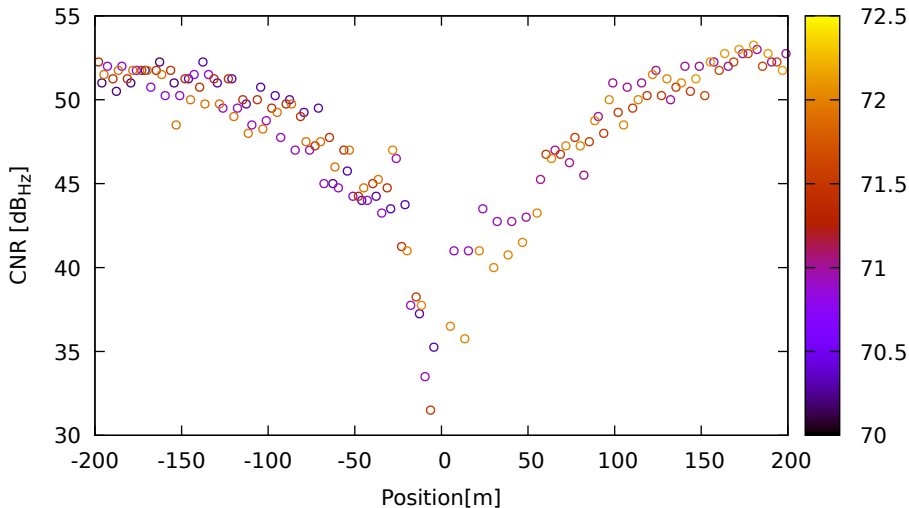
CNR vs position for G03 (L2) on LeicaGS18 - DOY 263 jam. 1
