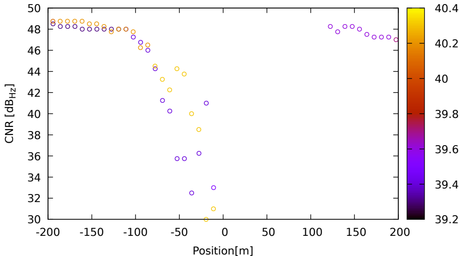
CNR vs position for G04 (L1) on LeicaGS18 - DOY 263 jam. 3
