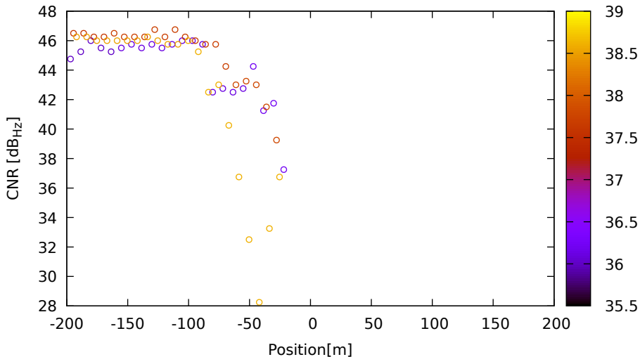
CNR vs position for G04 (L2) on LeicaGS18 - DOY 263 jam. 2
