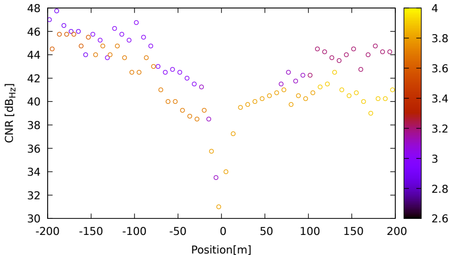
CNR vs position for G09 (L5) on LeicaGS18 - DOY 263 jam. 1
